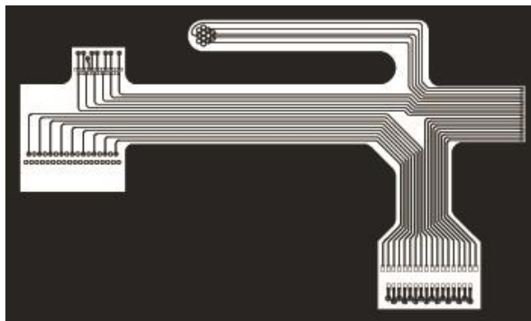
CAD-generated artwork
